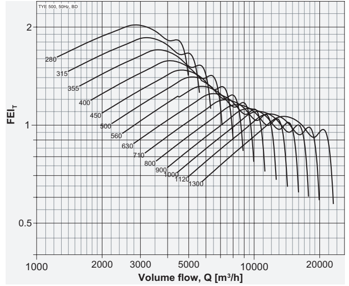
Model: TYE 500
