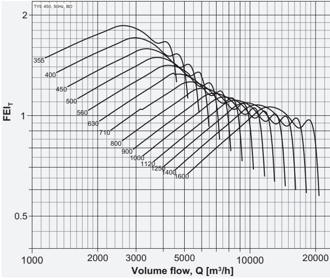
Model: TYE 450
