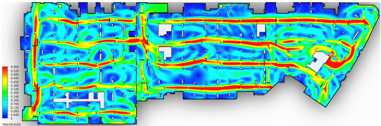
The high velocity air stream along the ceiling level will induce a low-velocity airstream at floor level, ensuring the required mixing of low-level and high-level atmosphere.
