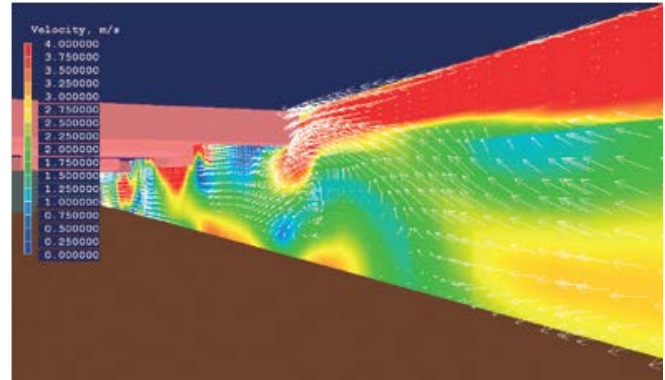
The high velocity air stream along the ceiling level will induce a low-velocity airstream at floor level, ensuring the required mixing of low-level and high-level atmosphere.
