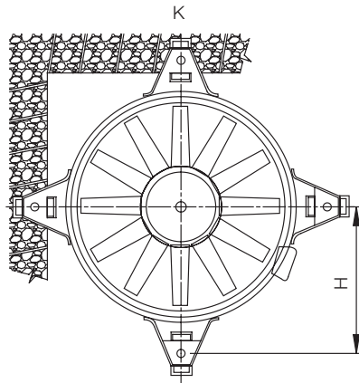
Figure 4b Square Platform Opening
