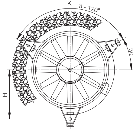
Figure 4a Circular Platform Opening
